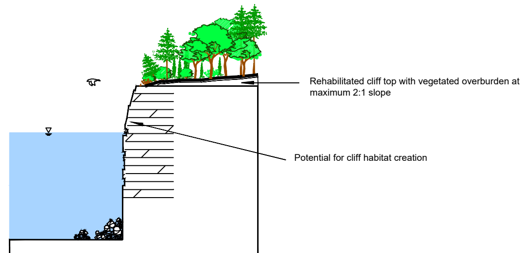
Figure 4.0 - Vertical Face
